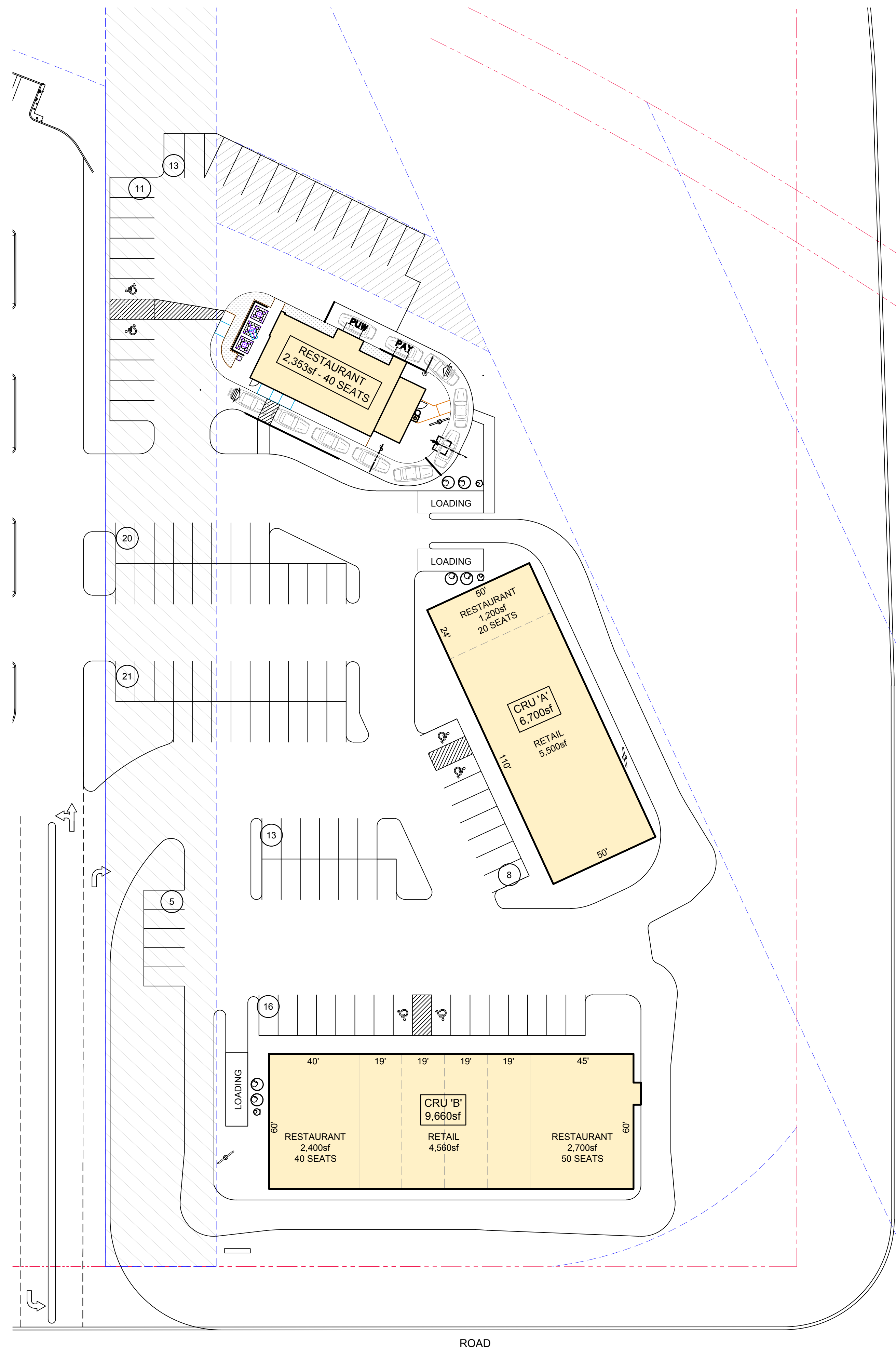
AVATEX COMMERCIAL SITE PLAN 1:350
